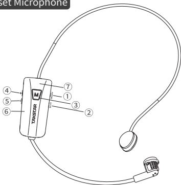
Headset microphone
